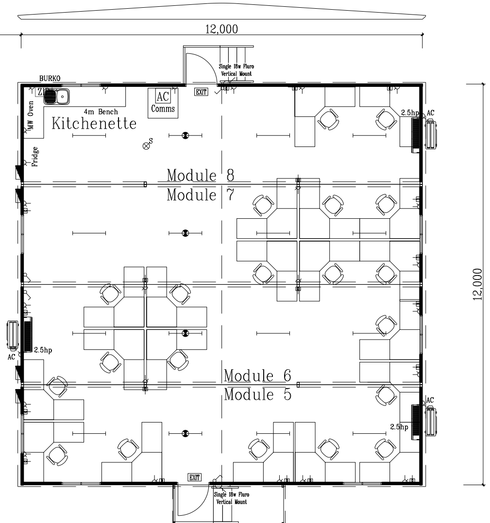
Modular Office a. 20 Workstations b. Kitchenette
