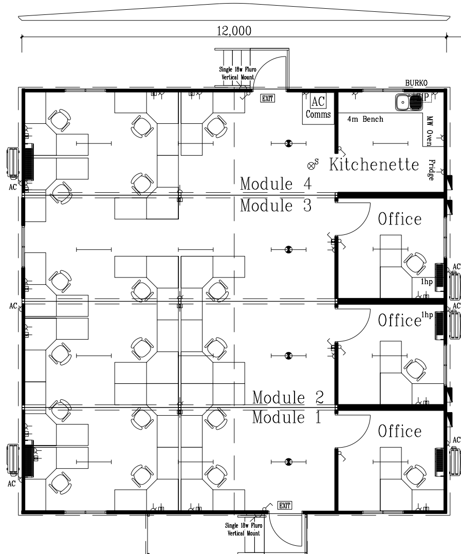
Modular Office a. 3 Closed Offices b. 17 Workstations c. Kitchenette
